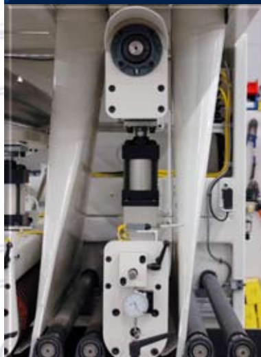
Shown with optional eccentric adjustment & dial indicator
